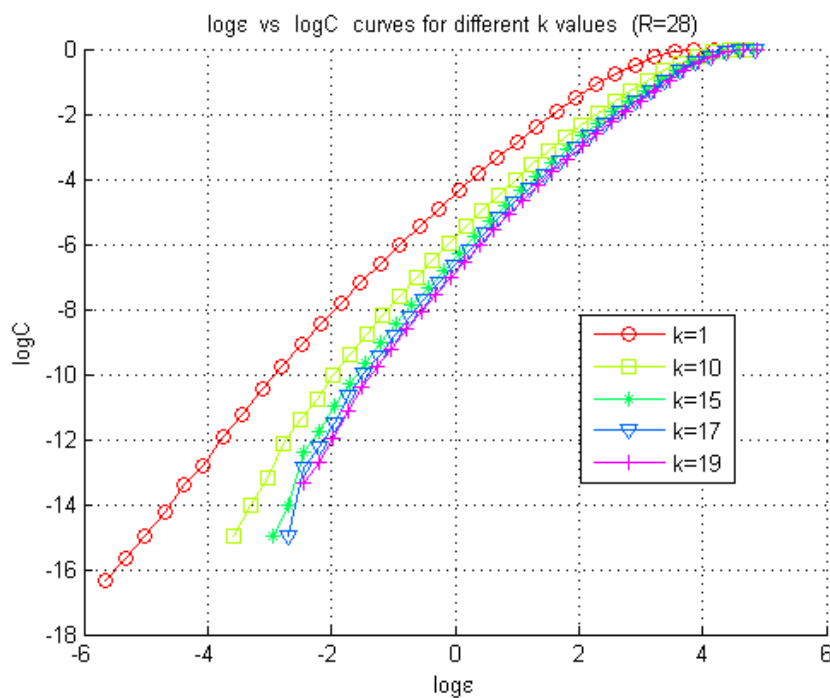
Figure 11. Exploration of the optimal radius for the KDE of a pdf using the Grassberger-Procaccia method. The figure illustrates the Correlation Sum (22) estimated at different radius values represented by \varepsilon for the Lorenz model in the chaotic regime ( R = 28 ).
