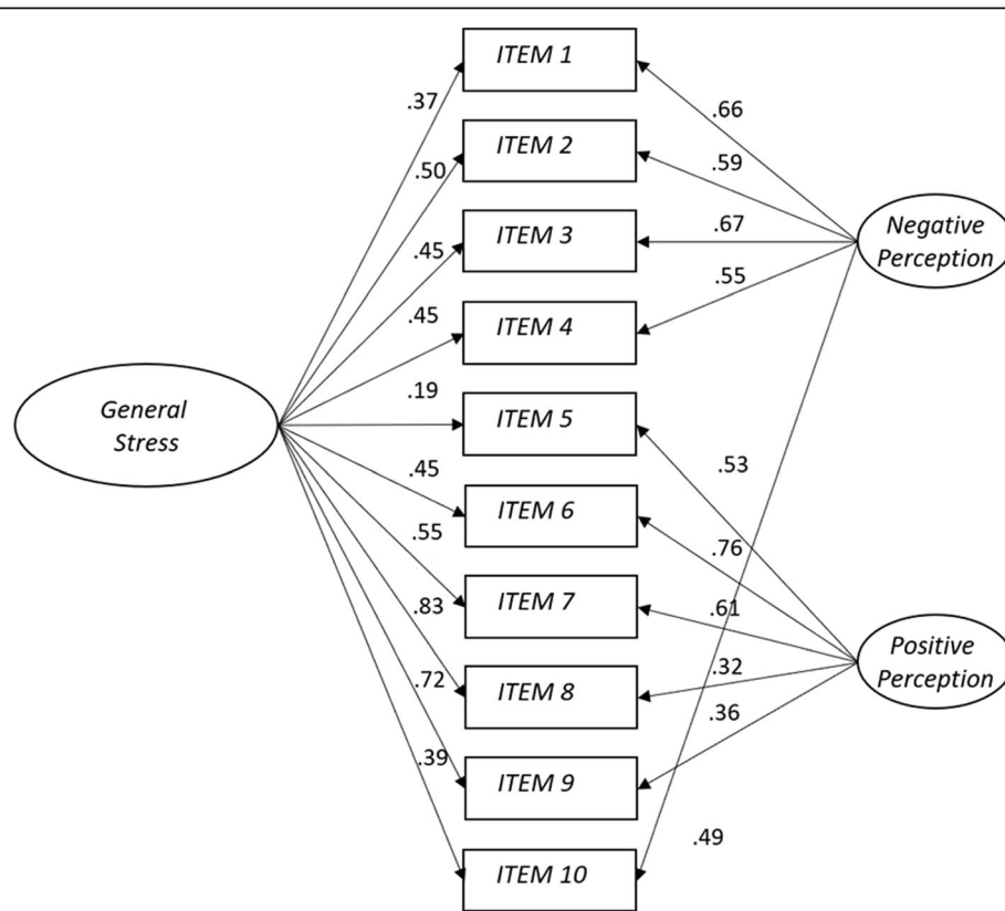
Fig. 1 The bifactor model with a general stress factor and two group factors
