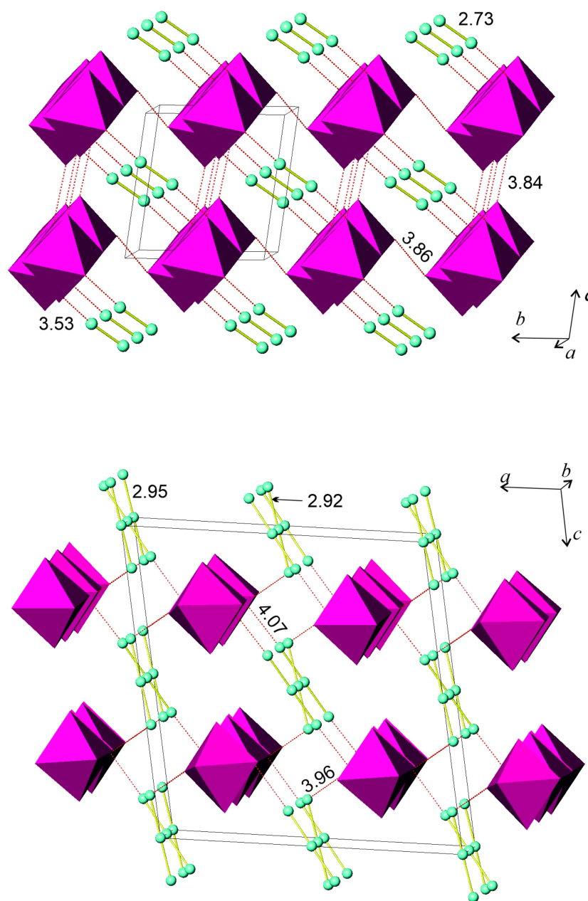
Figure 5. Patterns of I–I covalent (yellow, solid) and I...I intermolecular (red, dashed) interactions in the crystal structures of 3 (top) and 4 (bottom). Only iodine atoms (green) and [BiI 6 ] octahedra (purple) are shown. Interatomic distances are given in Å.
